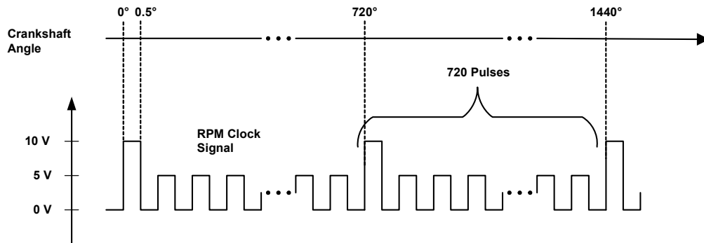
Abb. 8-4 RPM-Taktsignal
