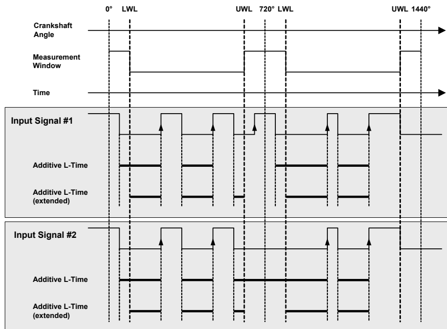
Abb. 33-26 Additive L-Time und Additive L-Time (extended)
