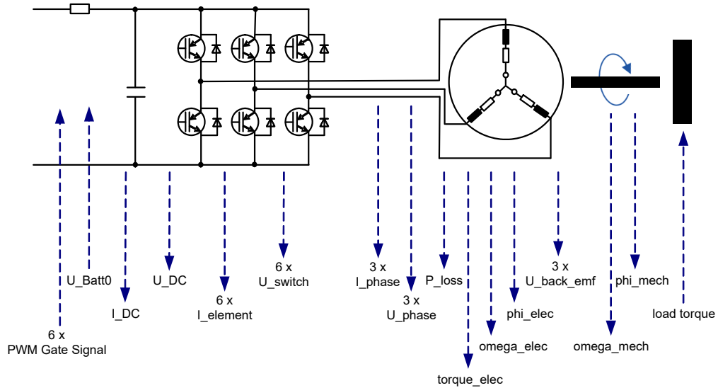
Abb. 23-54 Blockdiagramm des ES5340-PMSM-1.0.0 Modells
