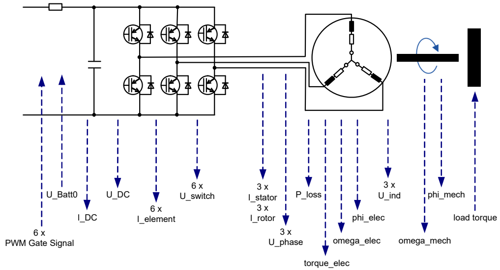
Abb. 23-60 Blockdiagramm des ES5340-IM-1.0.0 Modells
