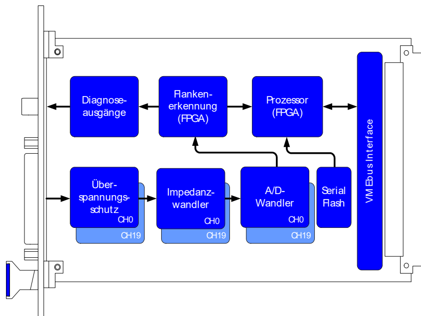
Abb. 12-1 Blockschaltbild des ES1336.1 Angle Synchronous Measurement Board
