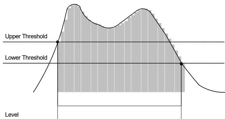
Abb. 12-4 Pulsintegration
