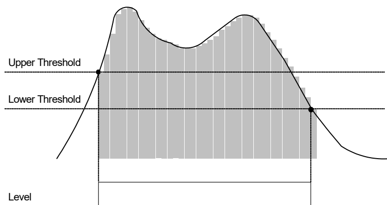
Abb. 11-4 Pulsintegration
