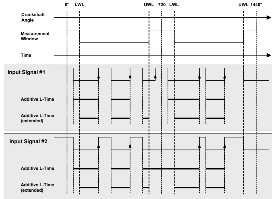
Abb. 32-26 Additive L-Time und Additive L-Time (extended)
