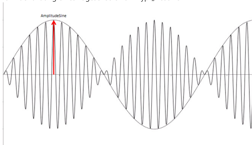
Abb. 22-44 Resolver: Sinuskanal
