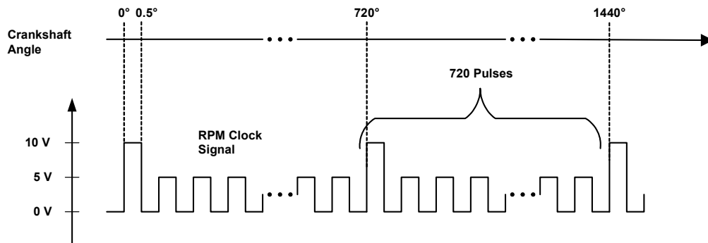
Abb. 7-4 RPM-Taktsignal
