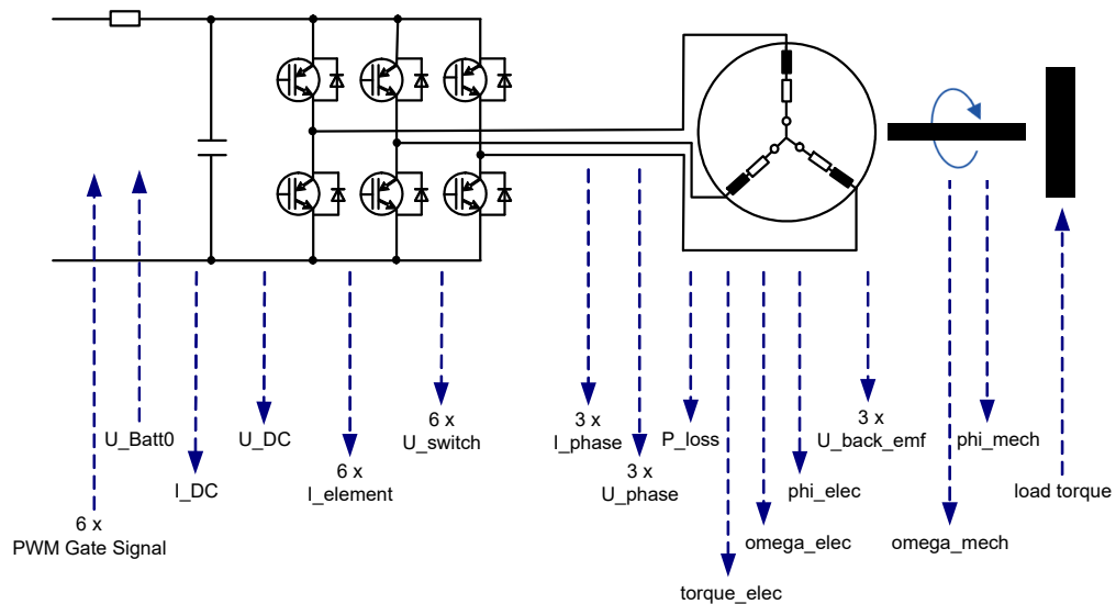
Abb. 22-54 Blockdiagramm des ES5340-PMSM-1.0.0 Modells
