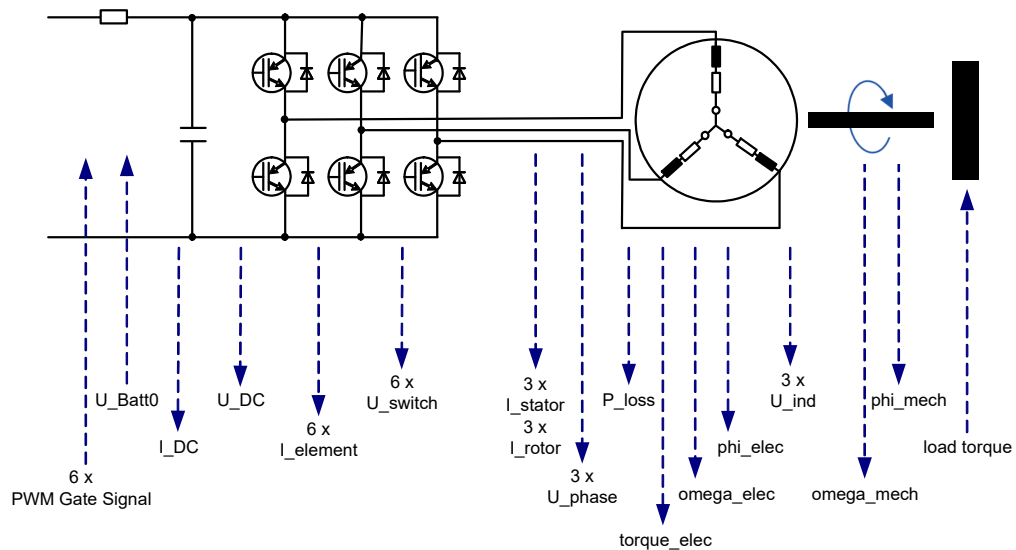
Abb. 22-60 Blockdiagramm des ES5340-IM-1.0.0 Modells
