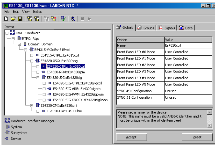
Abb. 17-6 Die Registerkarte „Globals“ des ES4320-CTRL Devices Front Panel LED #0 ... Front Panel LED #5 Mode
