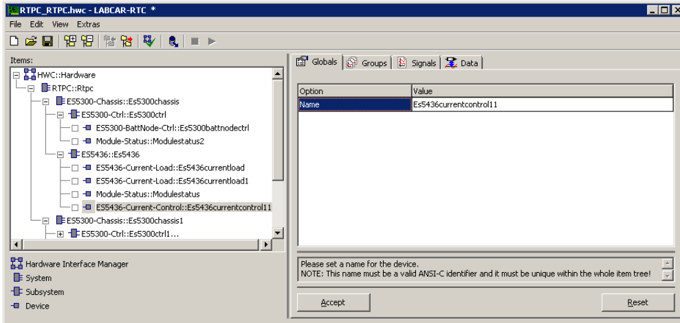
Abb. 27-8 Die Registerkarte "Globals" des ES5436-Current-Control-Device
