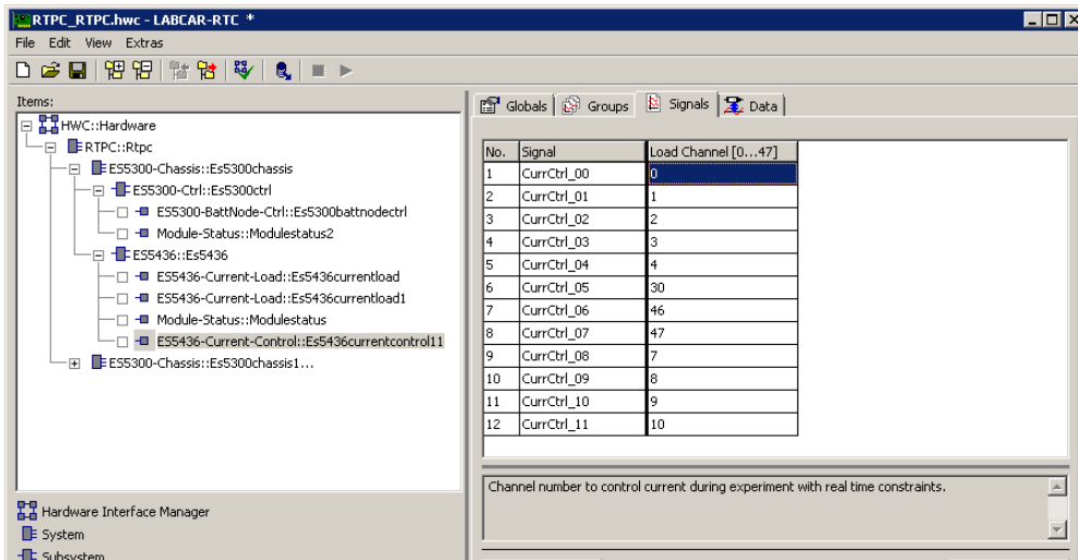
Abb. 27-10 Die Registerkarte "Signals" des ES5436-Current-Control-Device Load Channel [0...47]
