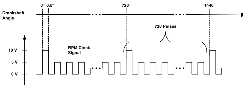
Abb. 7-4 RPM-Taktsignal
