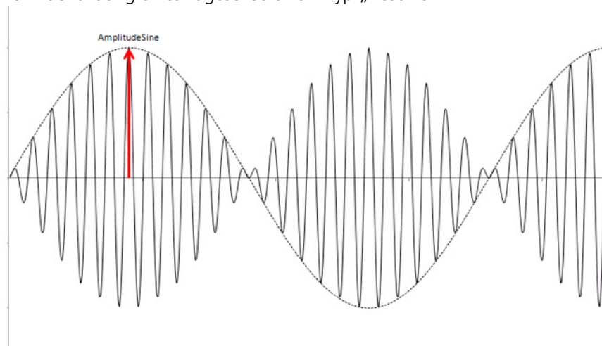
Abb. 22-43 Resolver: Sinuskanal
