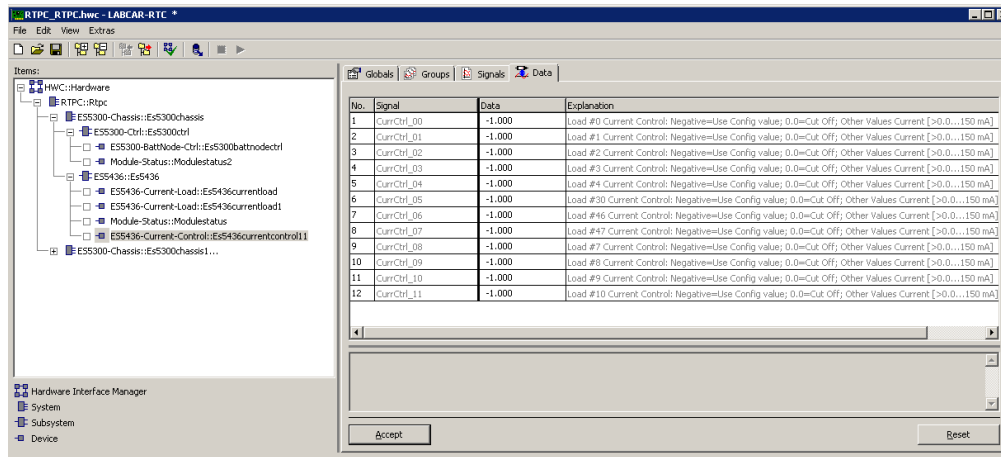
Abb. 27-11 Die Registerkarte "Data" des ES5436-Current-Control-Device
