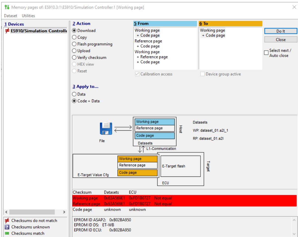
Image: Manage Memory Pages Dialog – showing Checksum not equal
