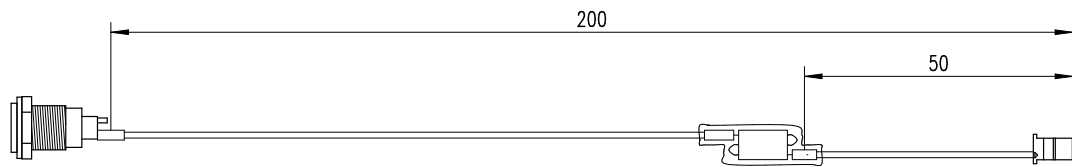
Figure 3: Mechanical Dimensions
