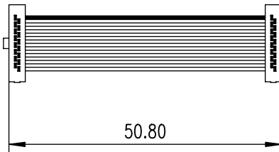
Fig. 2-3 ETAF5 Flatcable
