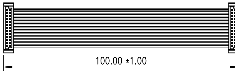
Figure 2: Measurement Drawing
