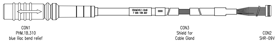
Figure 4 Connector Description
