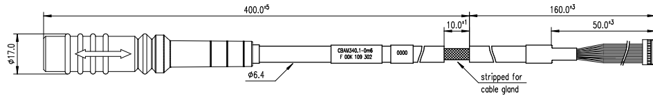
Figure 3 Mechanical Dimensions
