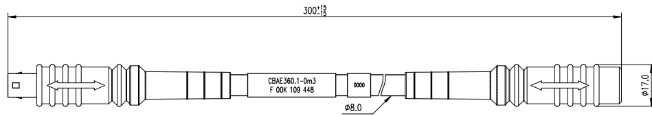
Figure 3 Mechanical Dimensions
