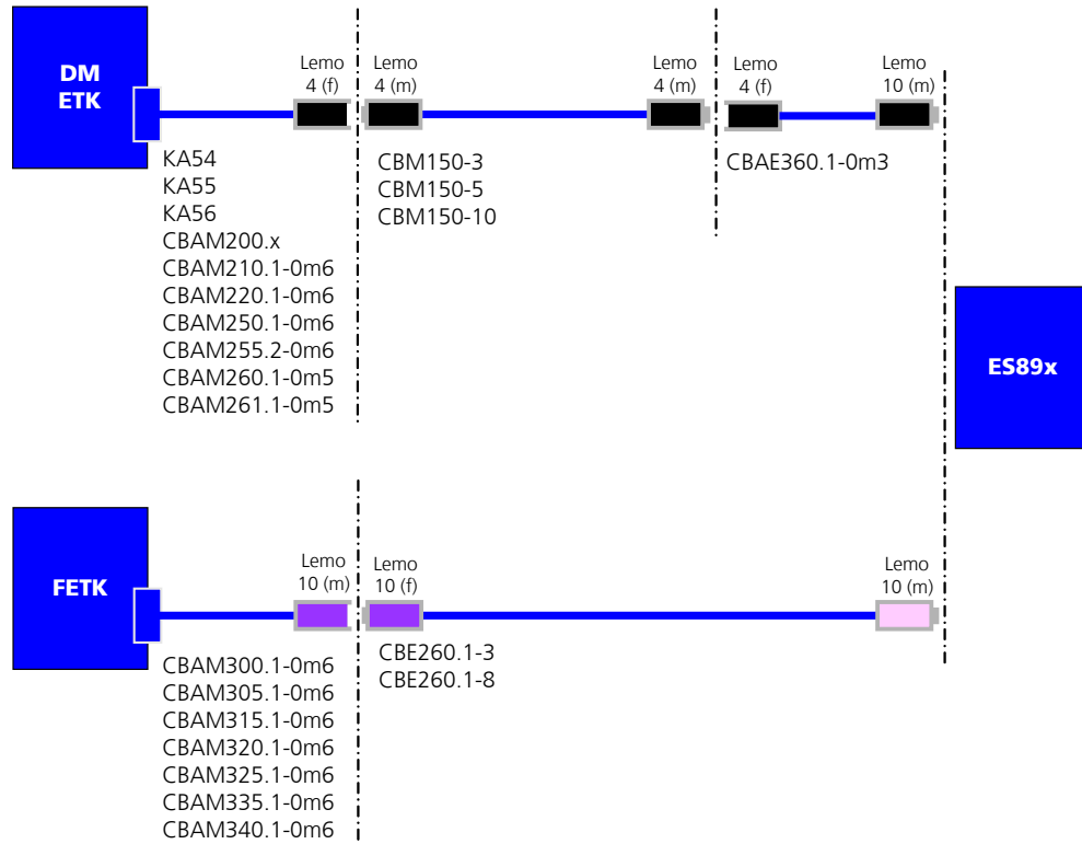
Figure 2 Cable Overview
